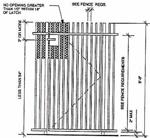
POOL GATE- RELEASE MECHANISM ALLOWED ON POOL SIDE ONLY
