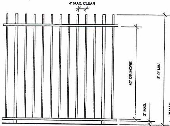
FENCE WITH HORIZONTAL MEMBERS AT MORE THAN 45" APART
