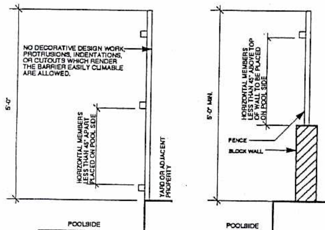
POOL- SIDE ELEVATION
