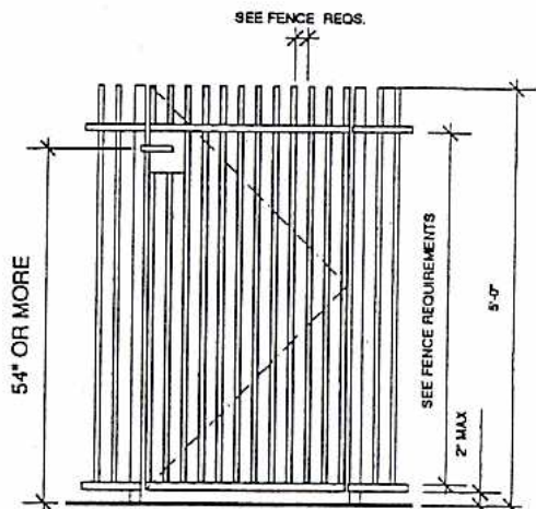
POOL GATE- RELEASE MECHANISM ALLOWED ON EITHER SIDE
