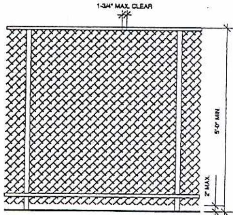
CHAIN LINK FENCE NOTES:
