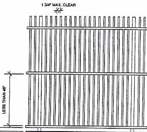
FENCE WITH HORIZONTAL MEMBERS AT LESS THAN 45" APART
