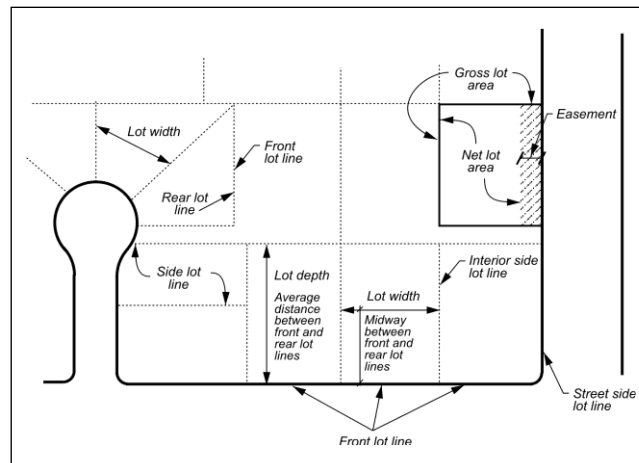
Figure 8-3 – Lot Types
