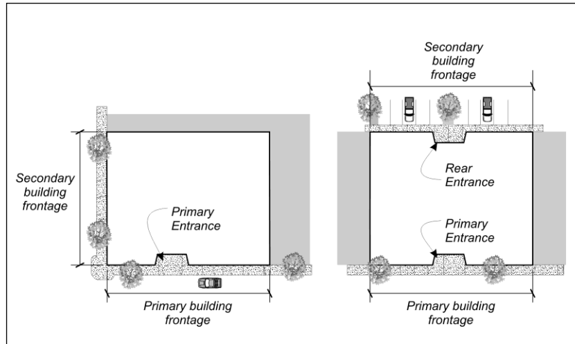
Figure 8-1 – Building Frontages
